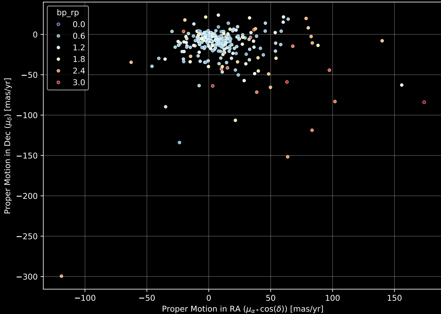
APOGEE DR17 Field: [sgr_tidal7] Proper Motion Diagram (n= 273)
