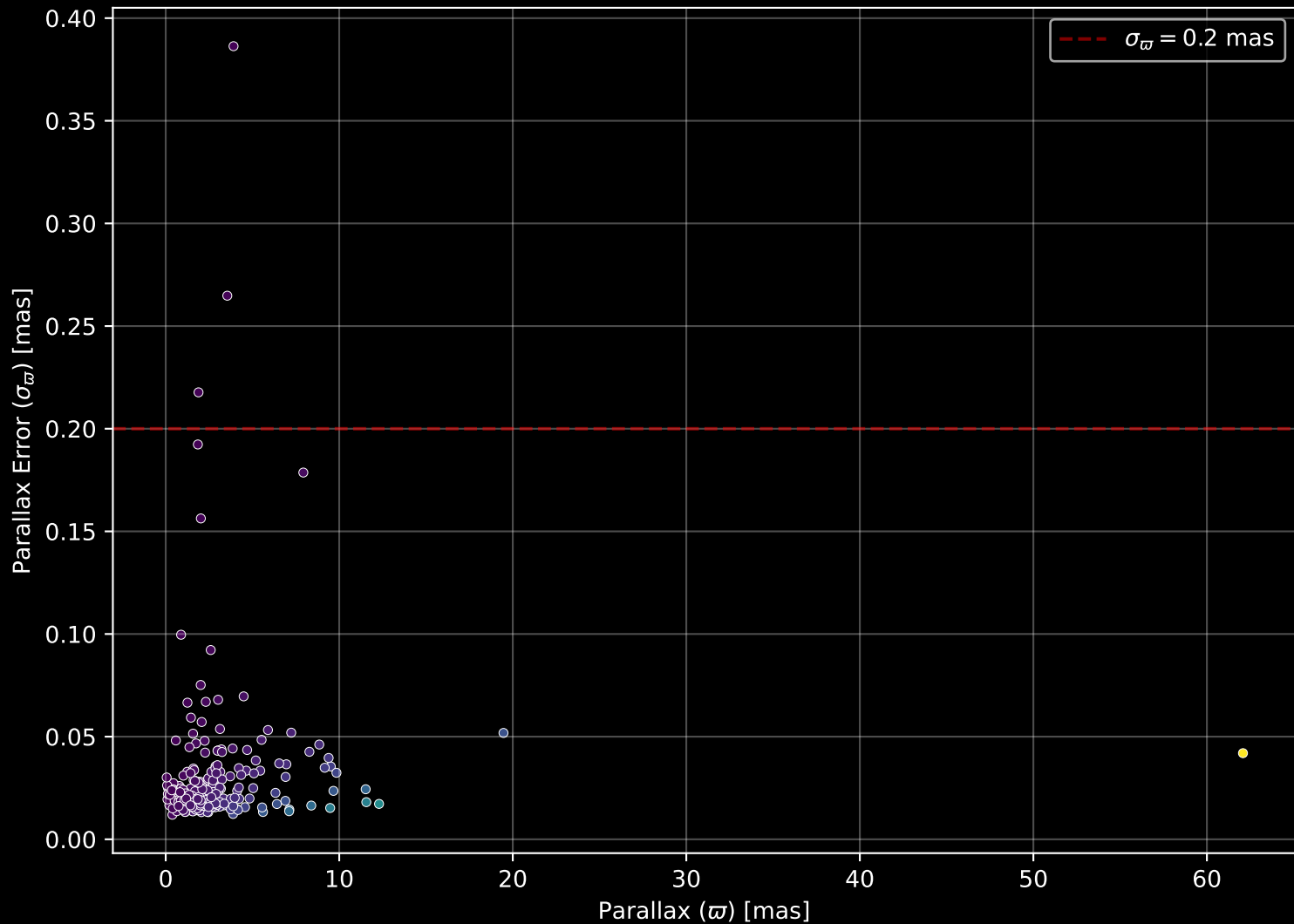
APOGEE DR17 Field: [sgr_tidal7] Parallax Quality (n= 273)
