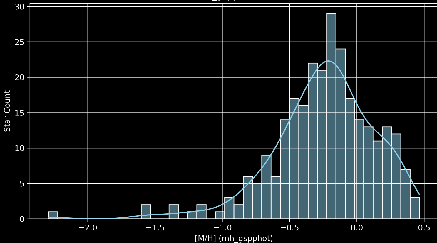
APOGEE DR17 Field: [sgr_tidal7 [M/H] (mh_gspphot) (n= 273)
