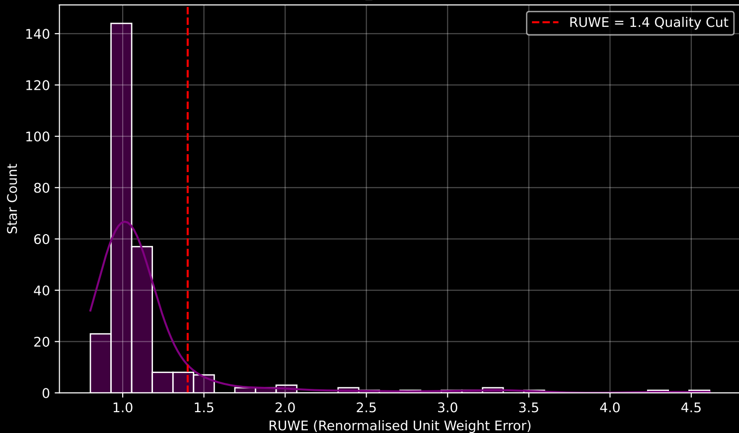
GAPOGEE DR17 Field [sgr_tidal7] RUWE Distribution (n= 265)
